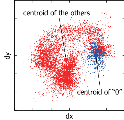
Figure 5. Distribution of the global feature vector selected at the first iteration for “0”-vs.-others classifier.
