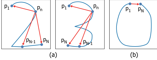
Figure 2. Potential of global features. (a): The local features around p_n do not have any discriminative power but the global features related to p_n do. (b): The global features can regulate the relationship between two widely separated points such as the starting and ending points.
