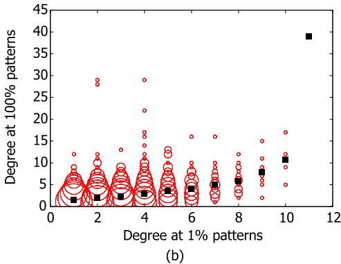
図4 パターン数の増加による次数の変化例 (■：平均). (a) Dataset 1 (活字), (b) Dataset 2 (手書き文字) Fig.4 Growth of Node degree with increase of the number of patterns. (■: average) (a) Dataset 1 (machine-printed patterns), (b) Dataset 2 (handwritten patterns).
