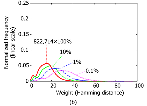
図5 エッジ重みと出現頻度の関係. (a) Dataset 1 (活字), (b) Dataset 2 (手書き文字) Fig.5 Distribution of edge weight. (a) Dataset 1 (machine-printed patterns), (b) Dataset 2 (handwritten patterns).
